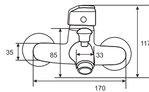
PROJECT Single Lever Bath Mixer Art # W5802
