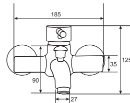
PRIDE Single Lever Bath Mixer Art # W7502
