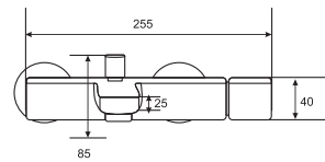
SLIM LINE Single Lever Bath Mixer Art # W7302
