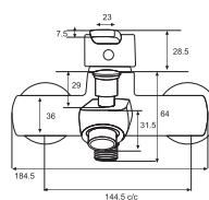
KIA Single Lever Bath Mixer Art # W7402
