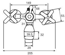
STAR Full Round Bath Mixer Art # W2502
