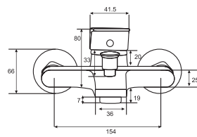
OPERA Single Lever Bath Mixer Art # W1102
