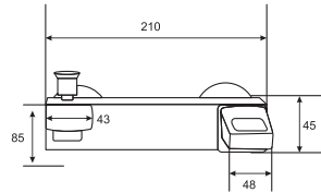
MARS Single Lever Bath Mixer Art # W7202
