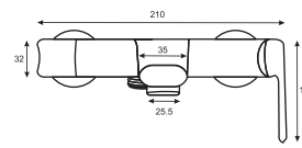
FAME Single Lever Bath Mixer Art # W1502
