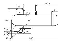
TECHNO Single Lever Bath Mixer Art # W9002
