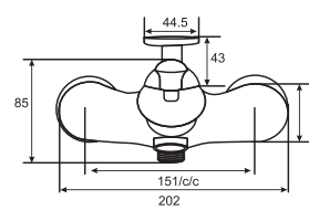
NOVIA Single Lever Bath Mixer Art # W5702
