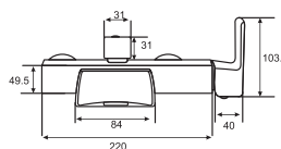
WATERFALL Single Lever Bath Mixer Art # W5402
