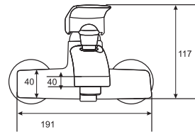
GRACE Single Lever Bath Mixer Art # W4602
