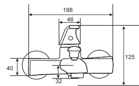
FLAT Single Lever Bath Mixer Art # W6702
