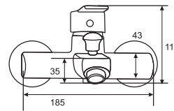
NEXT Single Lever Bath Mixer Art # W7802
