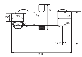
CASPER Single Lever Bath Mixer Art # W4902
