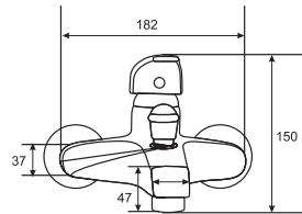
GEMINI Single Lever Bath Mixer Art # W3402
