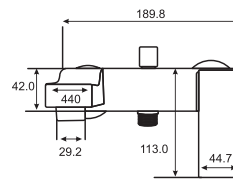
RECTA Single Lever Bath Mixer Art # W4802
